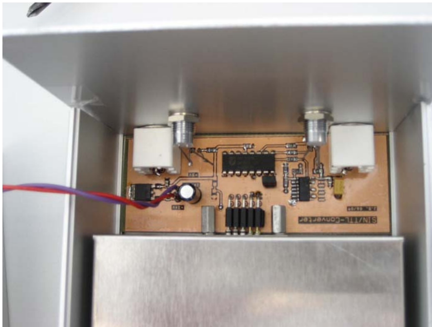
Figs.2: The upper photo shows the cabinet with its upper part containing the power supply removed showing the LPRO-unit with its metal shielding. All connections are via the small connector on the right side in the middle.
