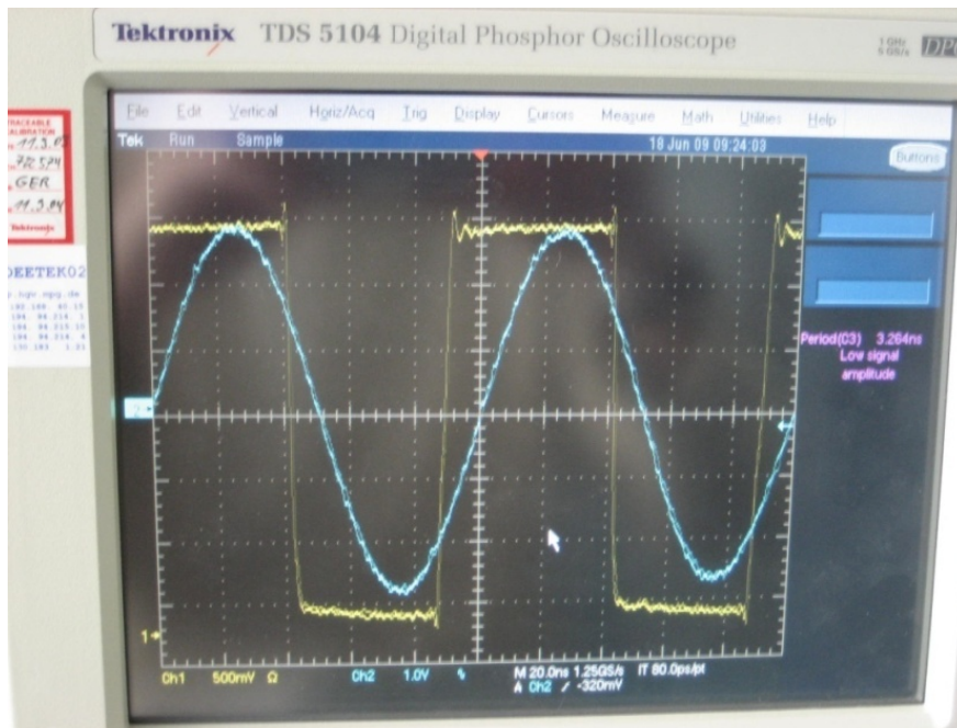
Fig.9: The two signals from the reference 10 MHz standard (blue) and the LPRO unit (yellow) are applied to an oscilloscope. The horizontal scale is 20ns per division. The sine wave is used to trigger the scope. The frequency deviation between the two signals is causing a time dependent phase shift between the two. By measuring the time for a 360 degrees phase shift the frequency deviation can be quantified. Typically almost 1000 seconds are measured for 360 degrees.
