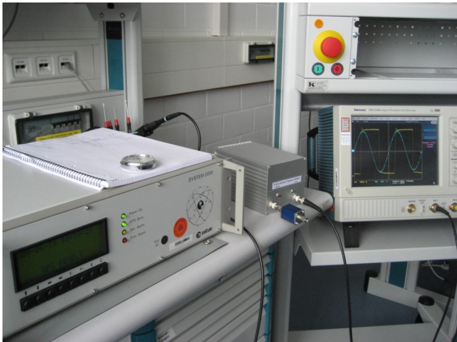
Fig.8: Test set-up comparing the 10 MHz signal from a GPS locked Rb-standard (left) with the signal delivered by the surplus unit described before (centre). Both signals are applied to an oscilloscope to compare frequencies by measuring their beat period.
